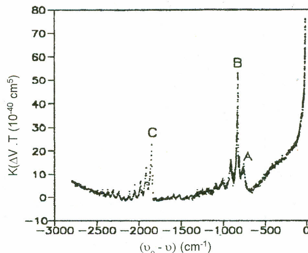
Fig 1. Expeyrmental blue wing profile of Cd line 326.1 nm (Helmi et al 1996 and Grycuk et al 1992).
