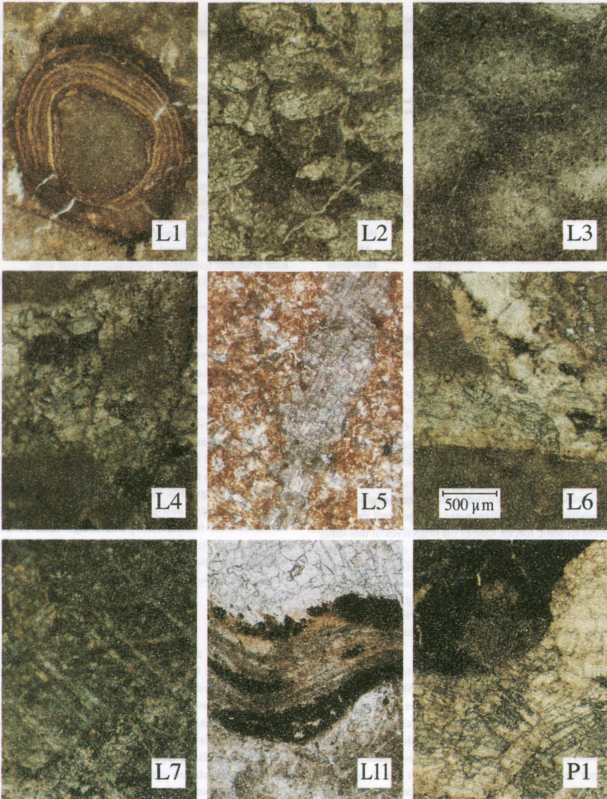
Fig. 3 Photomicrographs of Loralai formation and Parh limestone.
