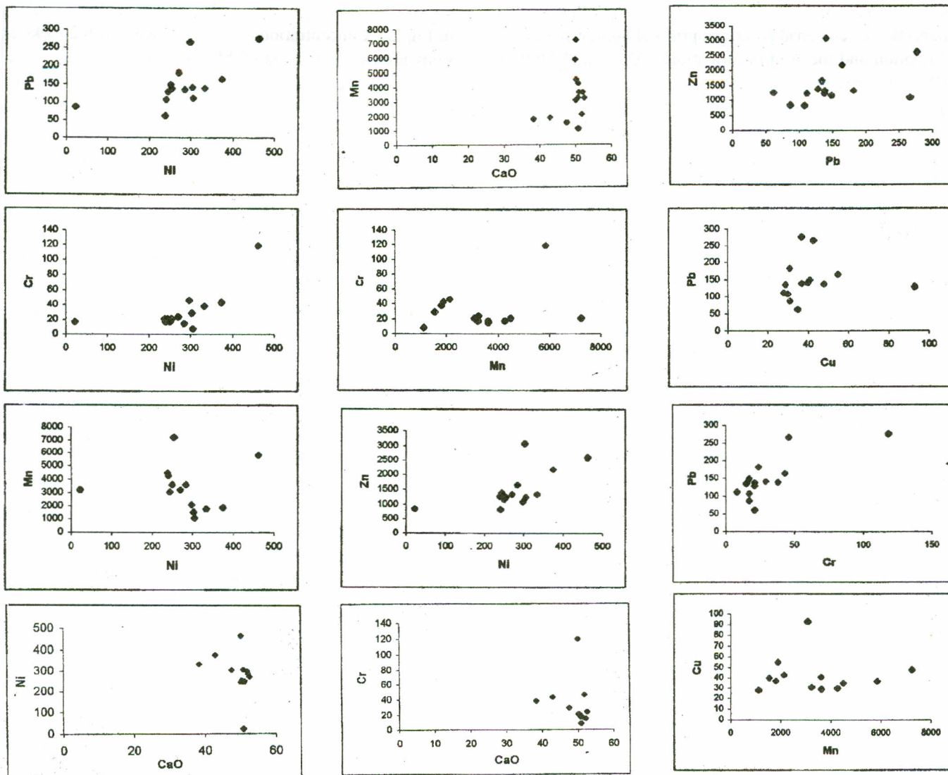
Fig. 2 Plots showing degree of correspondence between CaO with trace elements and degree of correspondence among different trace elements.
