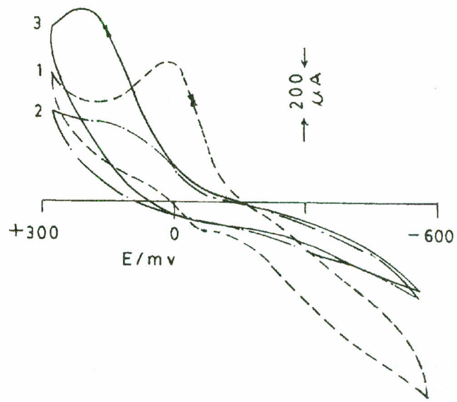
Fig 4c. Super imposed voltamogram of \text{Ni}_3\text{S}_2 electrode with the use of Ketx, Dtc and their mixtures at constant total concentration ( 5 \times 10^{-3} M) with varying mole ratios; potential sweep rate 30 \text{ msv}^{-1} .
