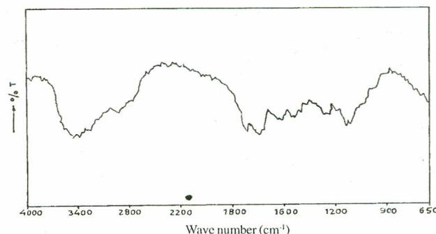
Fig 1. Spectrum of gelatin-g-MMA.
