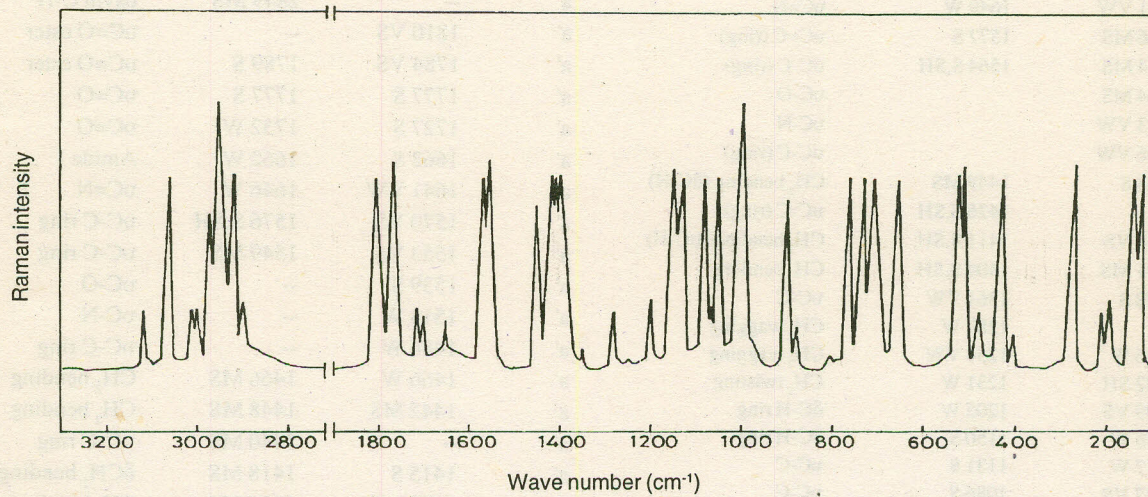
Fig 3a. Laser Raman spectrum of SPDP.
