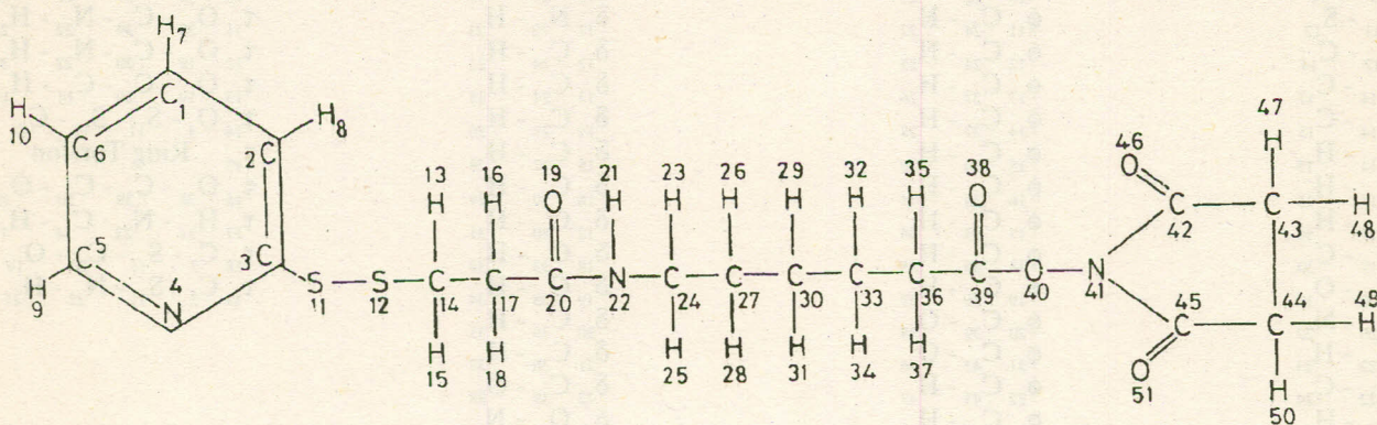
Fig 1b. Structure of LC - SPDP.
