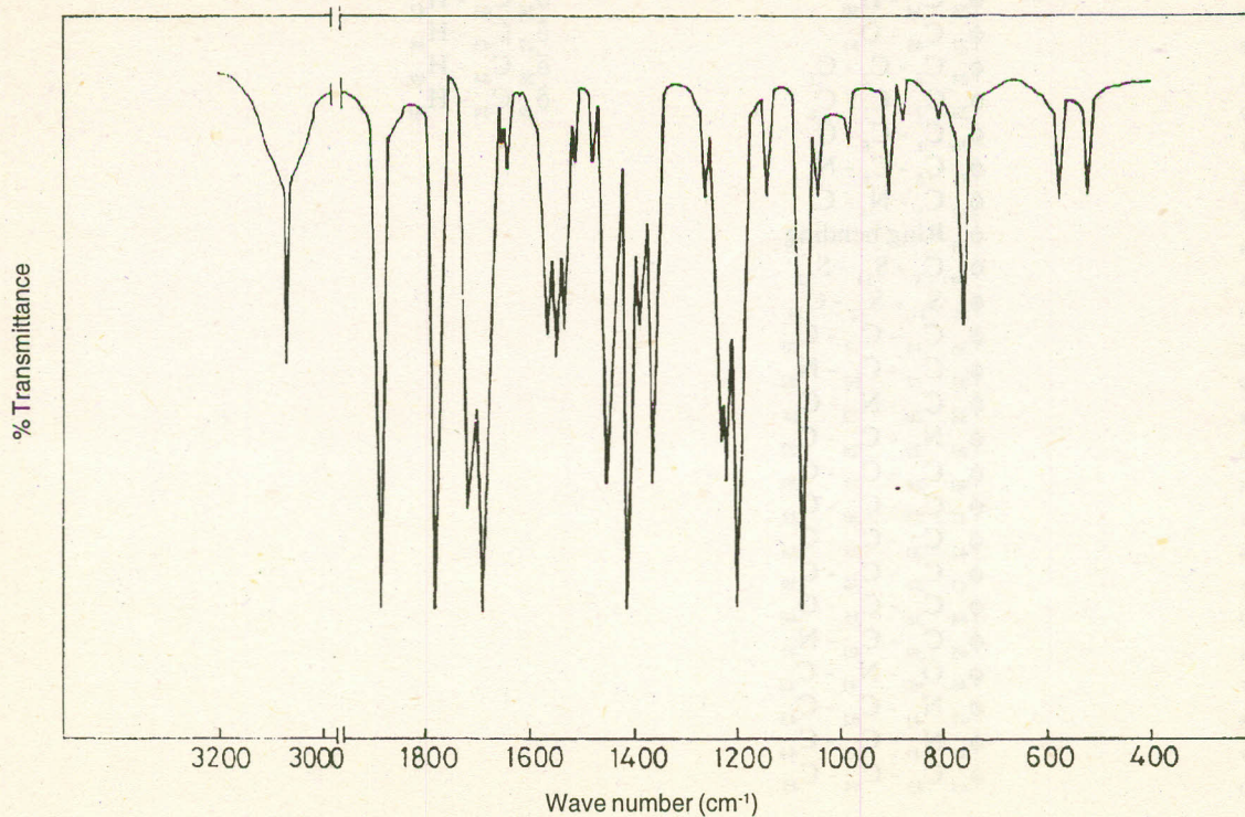
Fig 2a. FTIR spectrum of SPDP.
