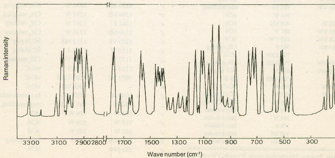
Fig 3b. Laser Raman spectrum of LC - SPDP.
