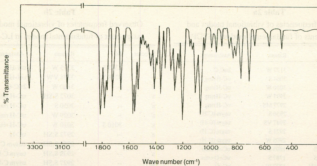
Fig 2b. FTIR spectrum of LC - SPDP.
