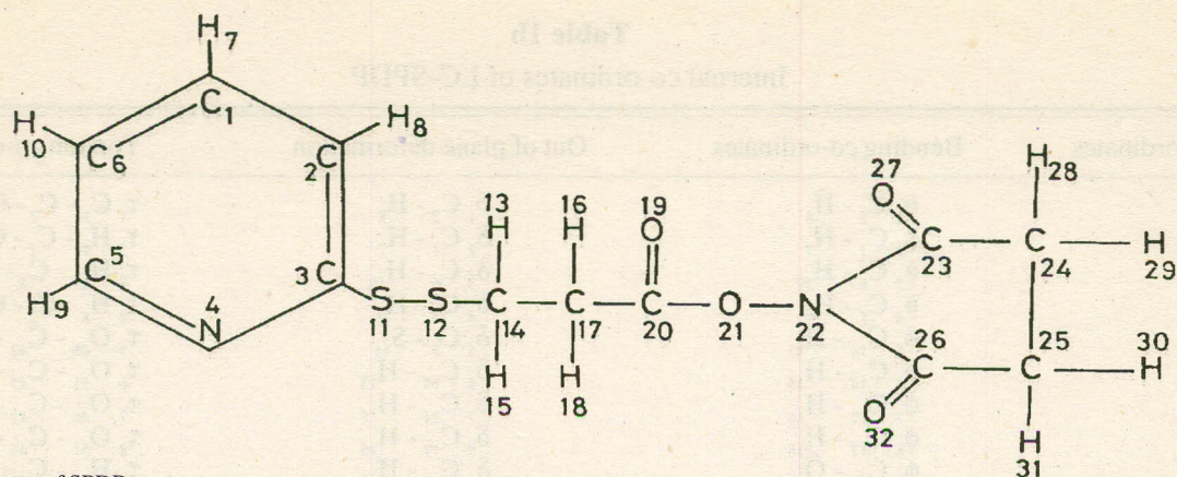
Fig 1a. Structure of SPDP.
