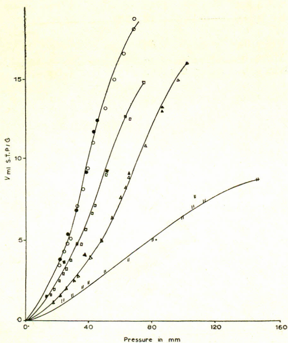
Fig. 4.—Adsorption of methanol on carbon black. O at 25°, □ at 30°, △ at 35°, || at 40°.
