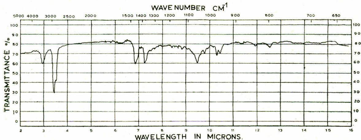
Fig. 2.—Showing Infra-red Spectra of Compound B.
